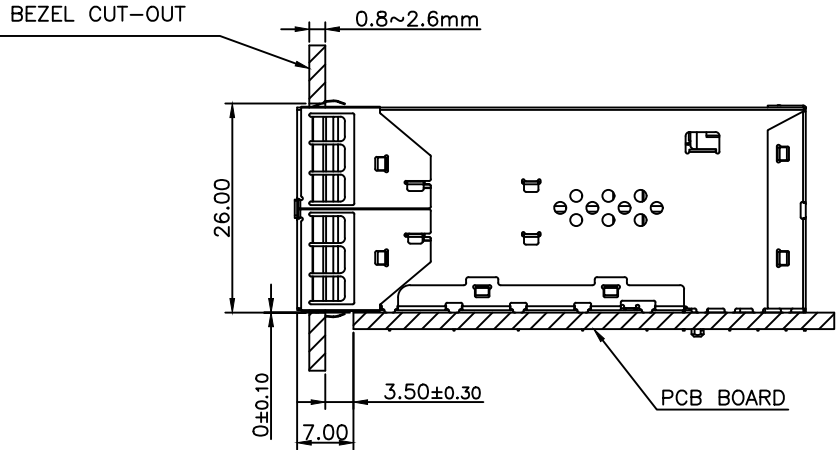
BEZEL CUT-OUT CENTER SPACING DETAIL BEZEL THICKNESS:0.8-2.6
